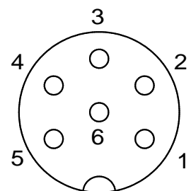
6pol / 240°
