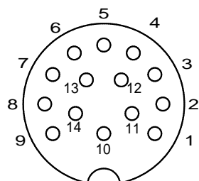
14pol / 240°
