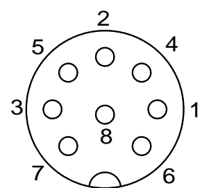
8pol / 270°
