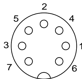
7pol / 270°
